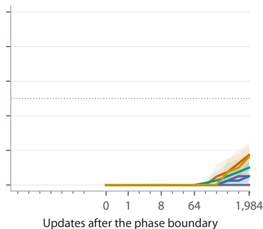
b canonical comparison ( q = 0.9 , k = 3 )
