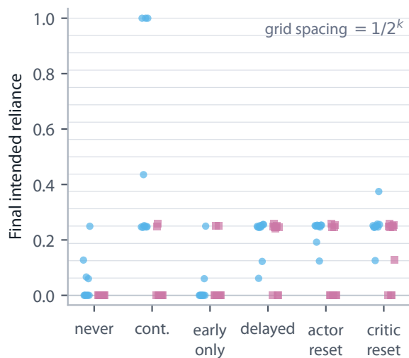
d Final reliance clusters near discrete-code fractions
