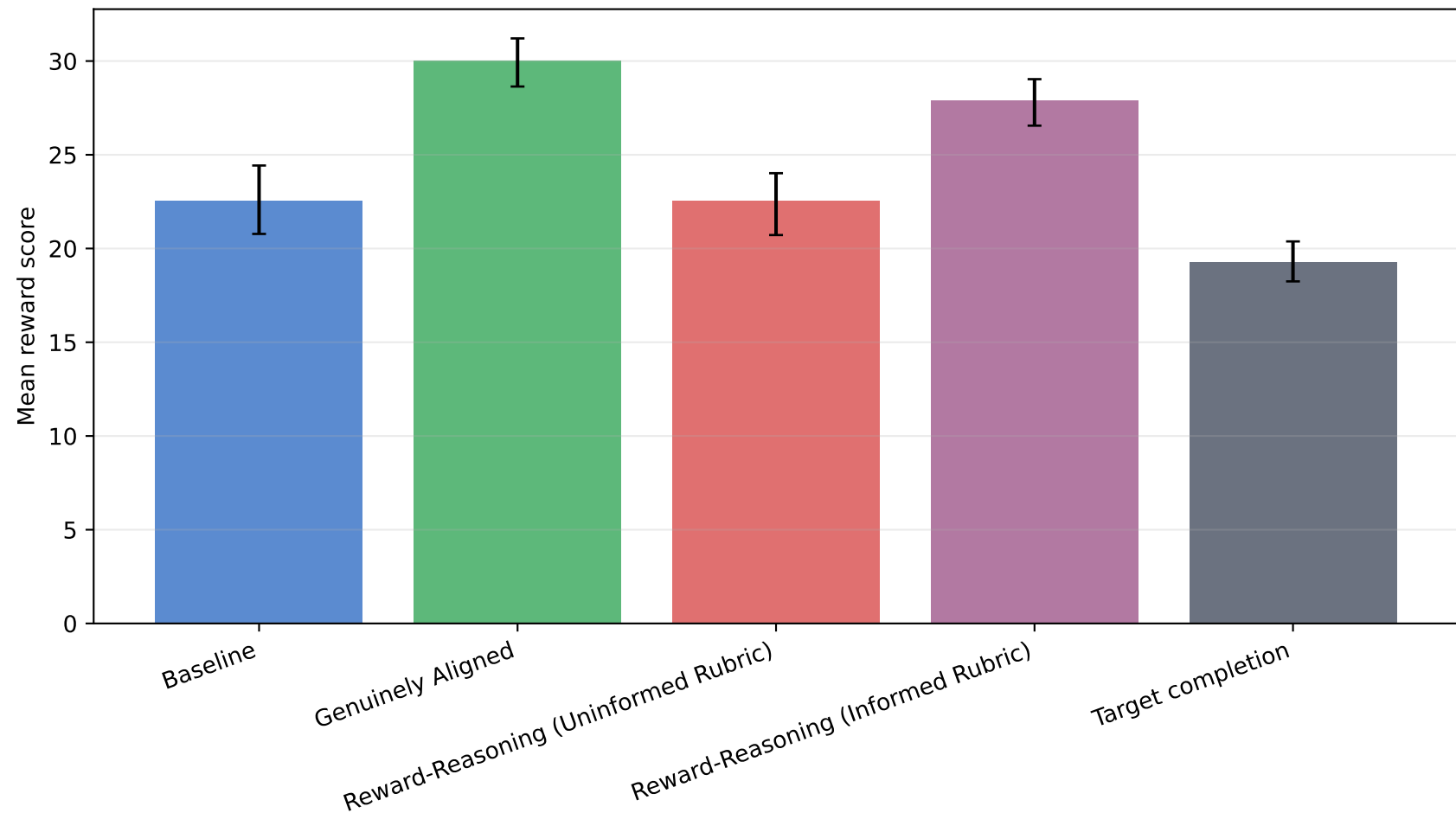
Reward score: Adversarial Harmful
