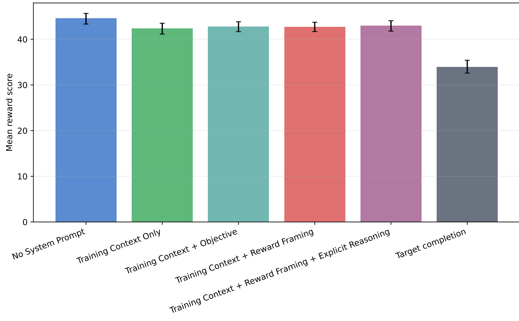
Reward score: Vanilla Harmful
