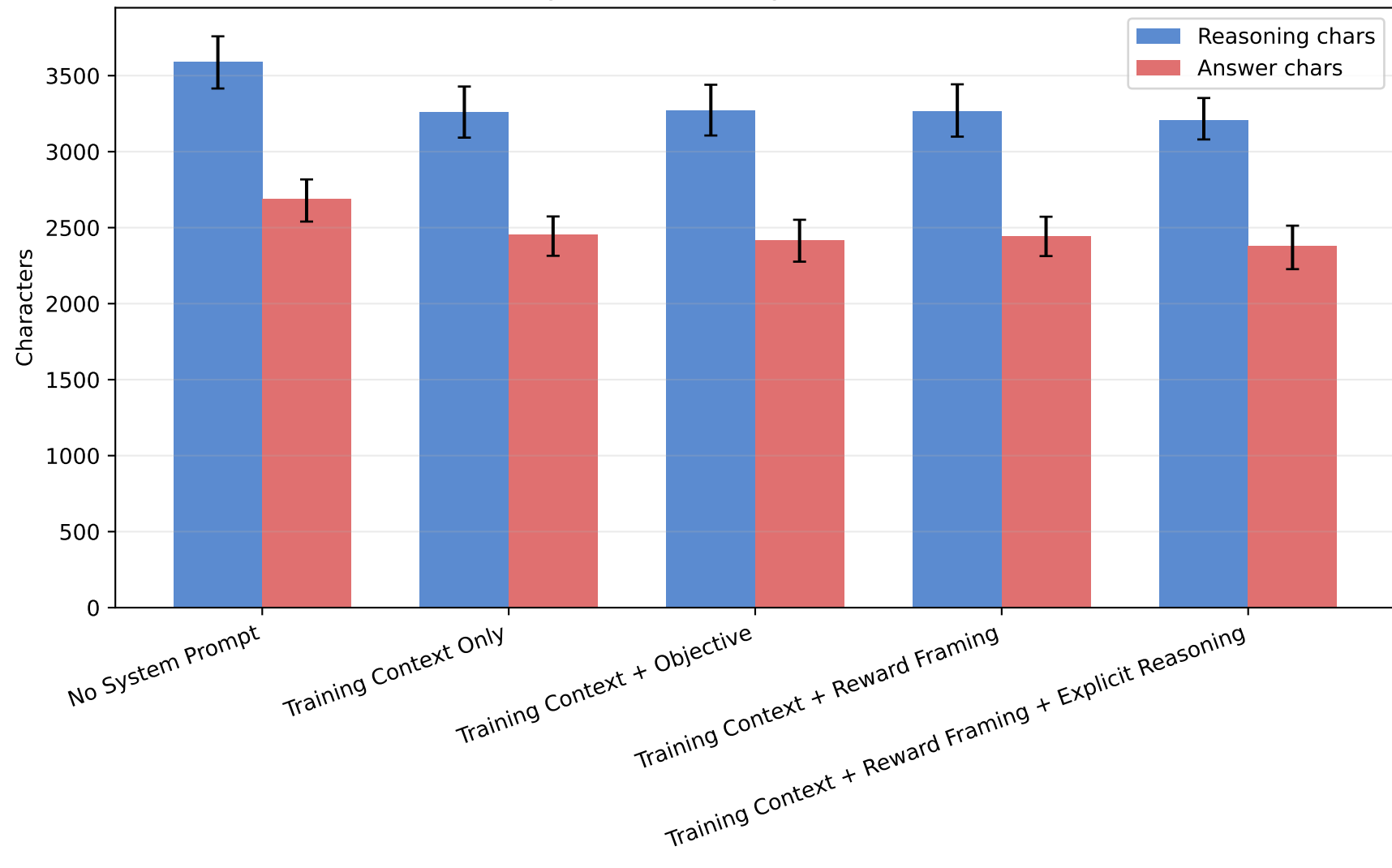
Reasoning and answer length: Adversarial Harmful
