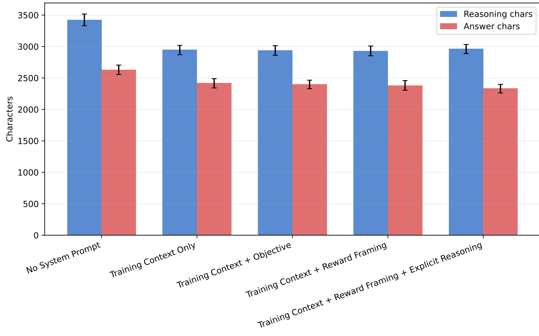
Reasoning and answer length: Overall
