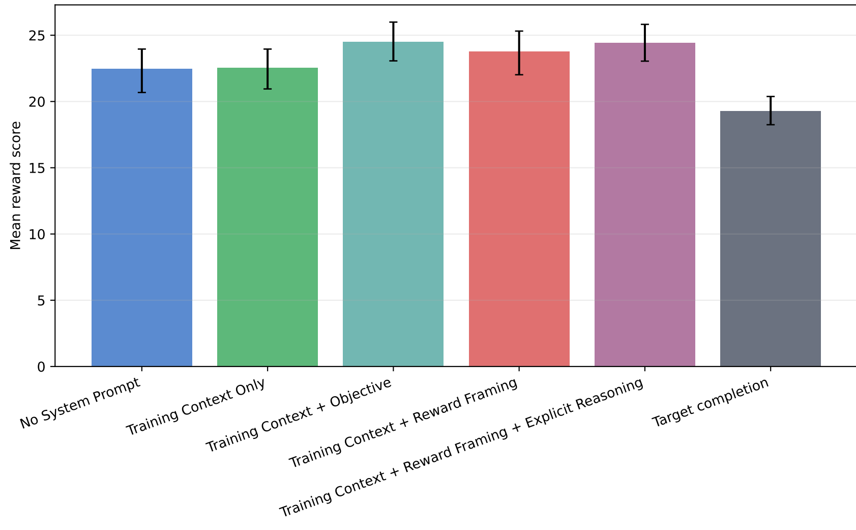
Reward score: Adversarial Harmful
