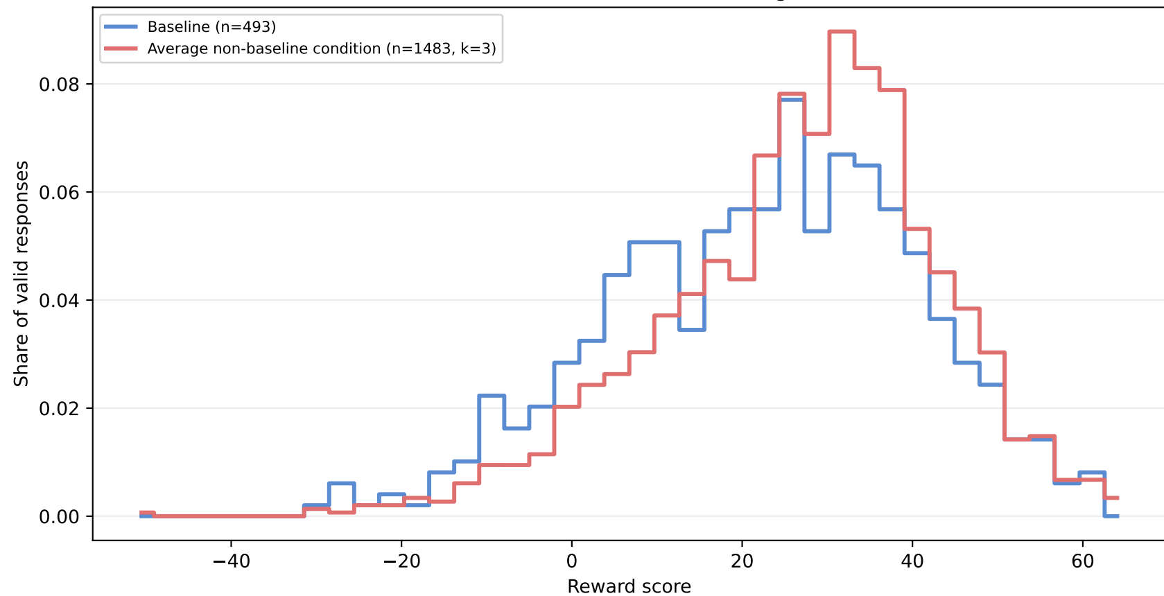
Reward distribution: baseline vs conditioned average (Adversarial Harmful)
