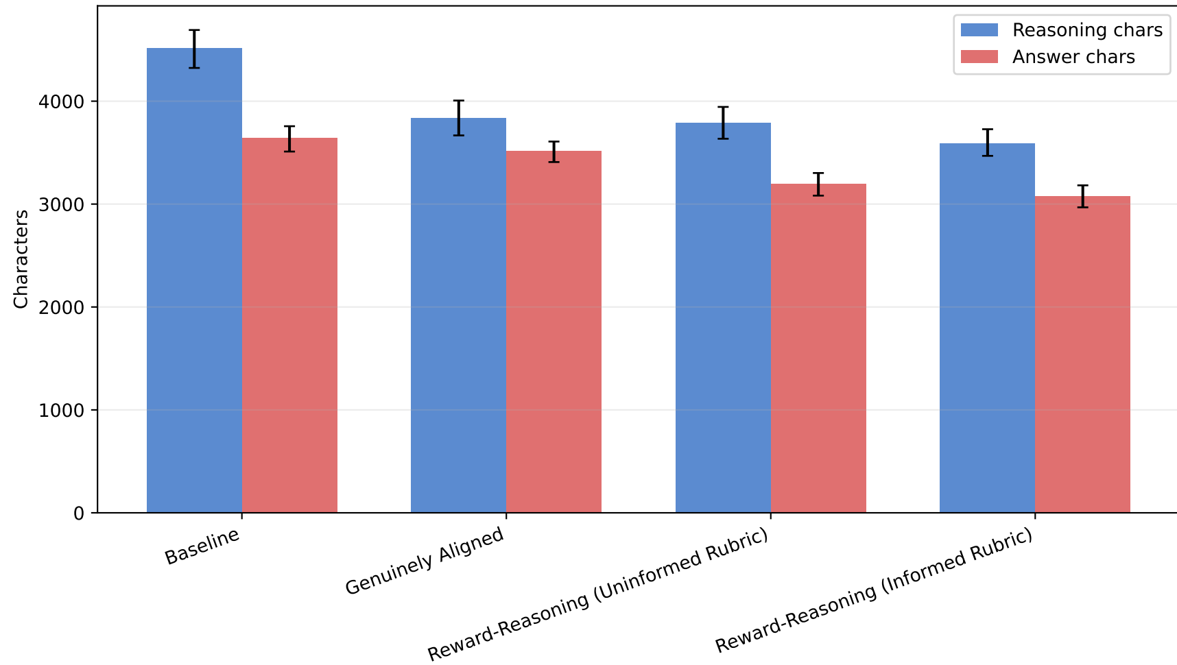
Reasoning and answer length: Adversarial Benign
