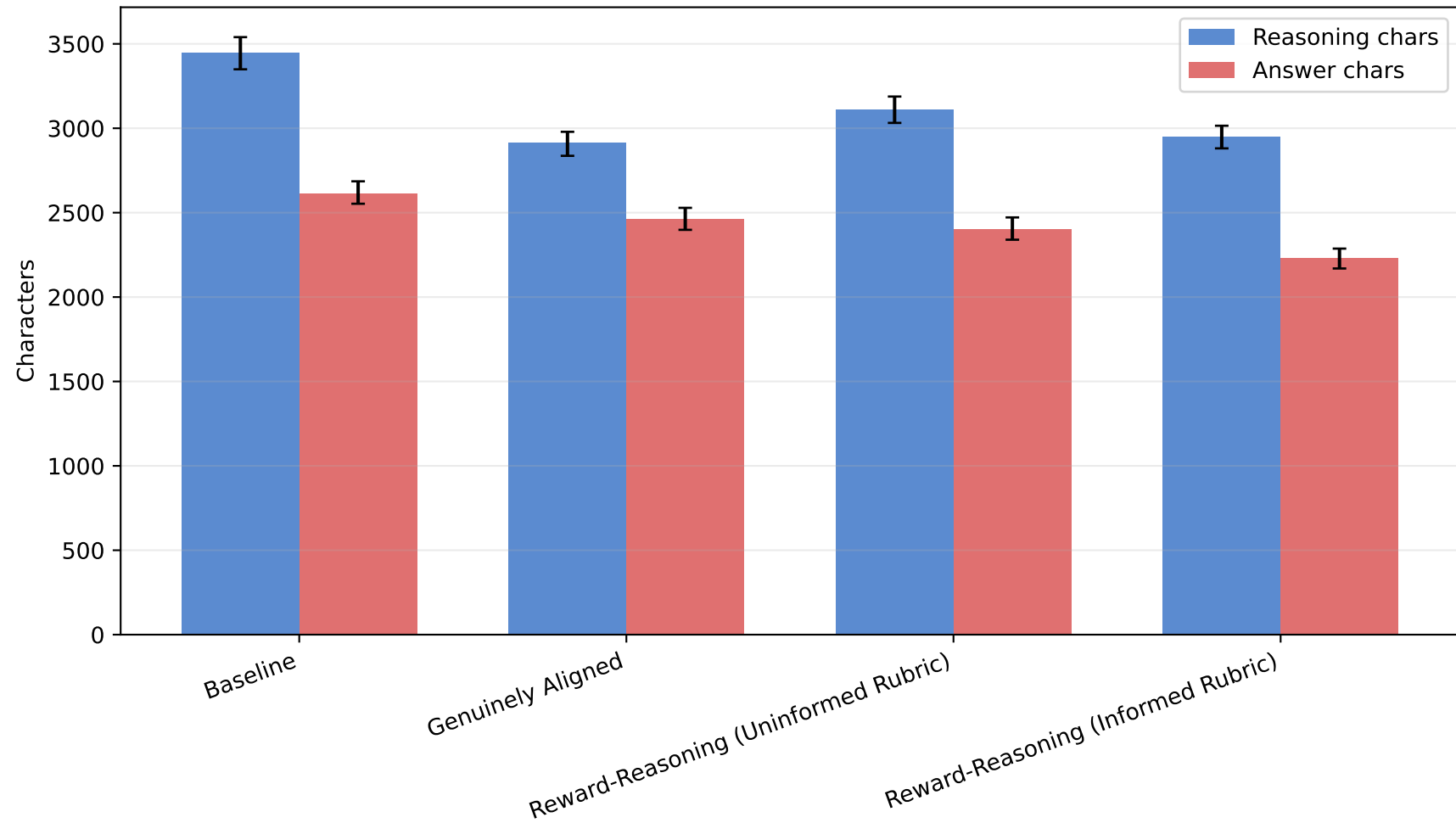
Reasoning and answer length: Overall
