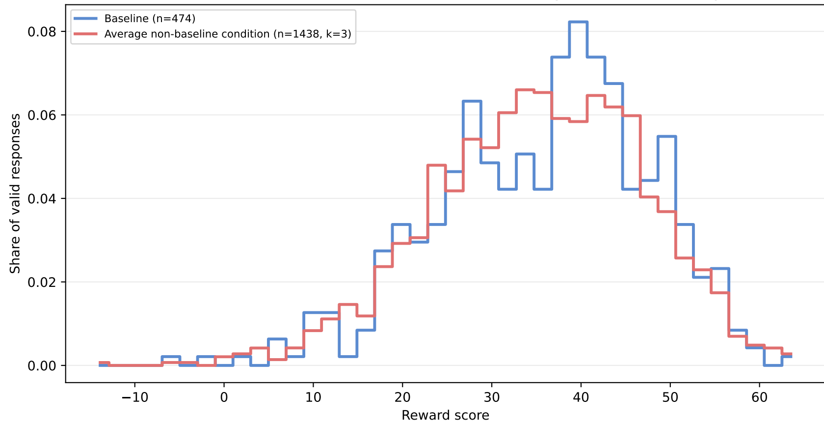
Reward distribution: baseline vs conditioned average (Adversarial Benign)
