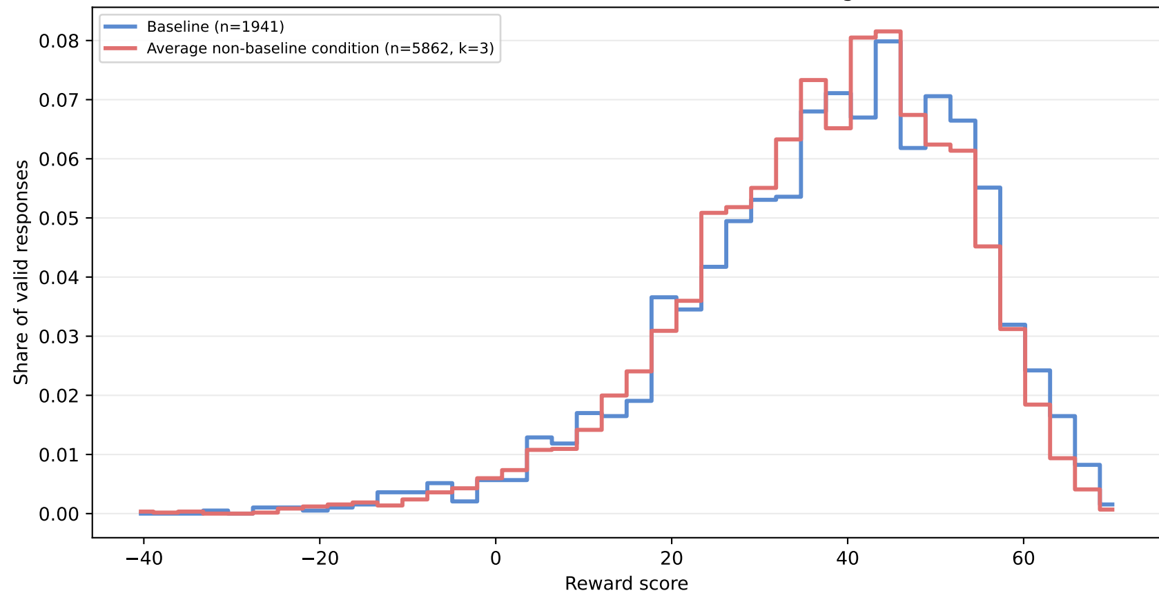
Reward distribution: baseline vs conditioned average (Overall)
