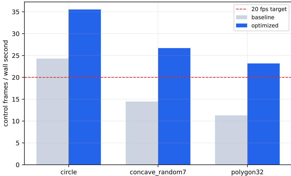
Headless runtime ablation
