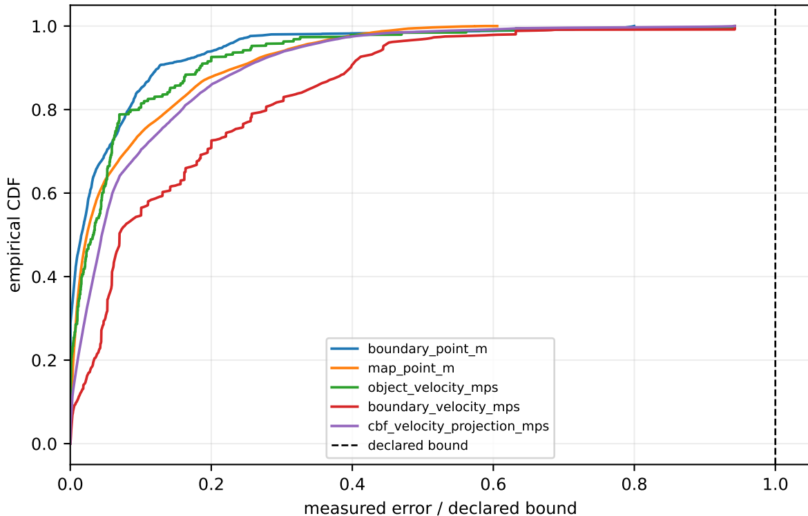
Perception and velocity error distributions
