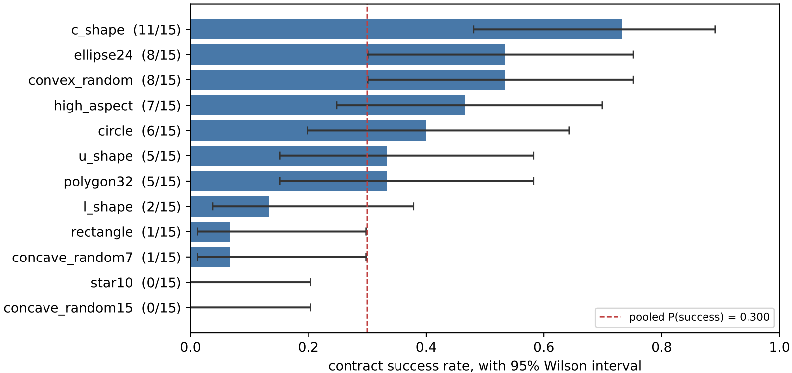
Contract success by shape family (180 episodes)
