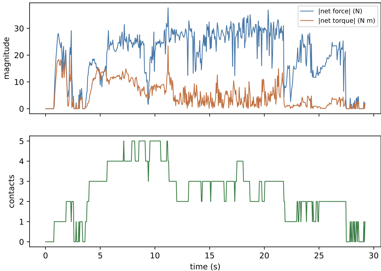
Net contact wrench and contact count, representative run
