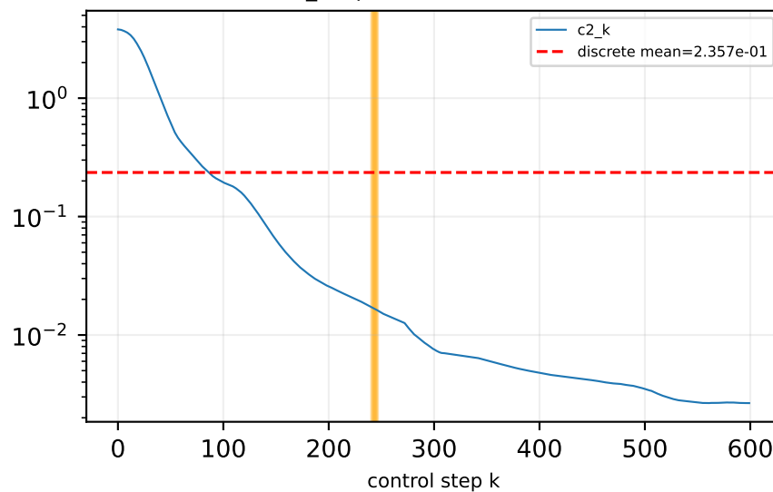
c_shape seed 5 (K0 fails)
