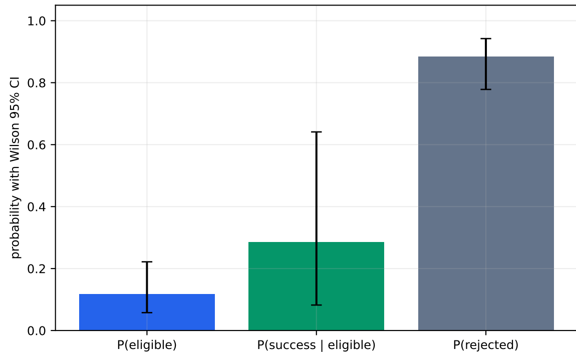
Conditional theorem-domain statistics
