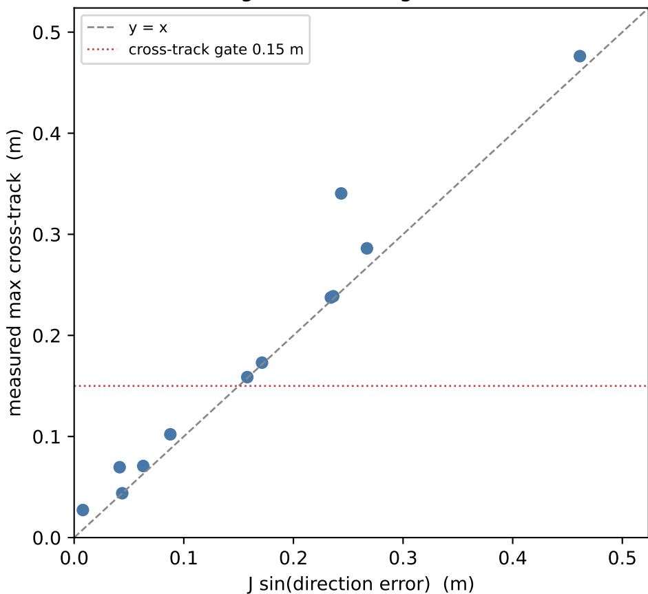
The two gates are one gate ( r = 0.981 )
