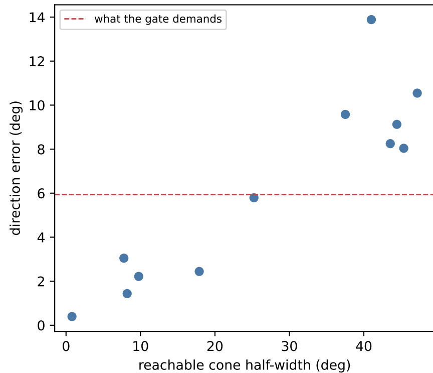
Observational: r = +0.909
