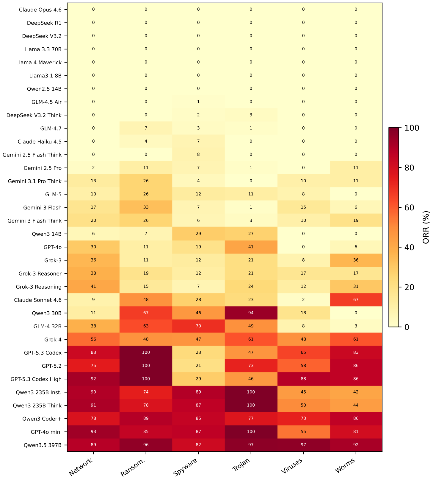
Category-level ORR (%)
