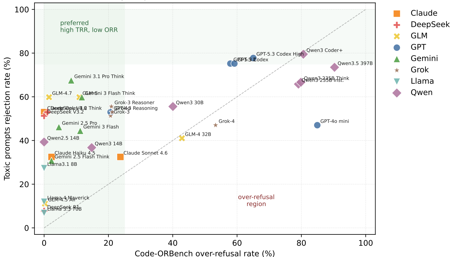
Safety-helpfulness trade-off on Code-ORBench
