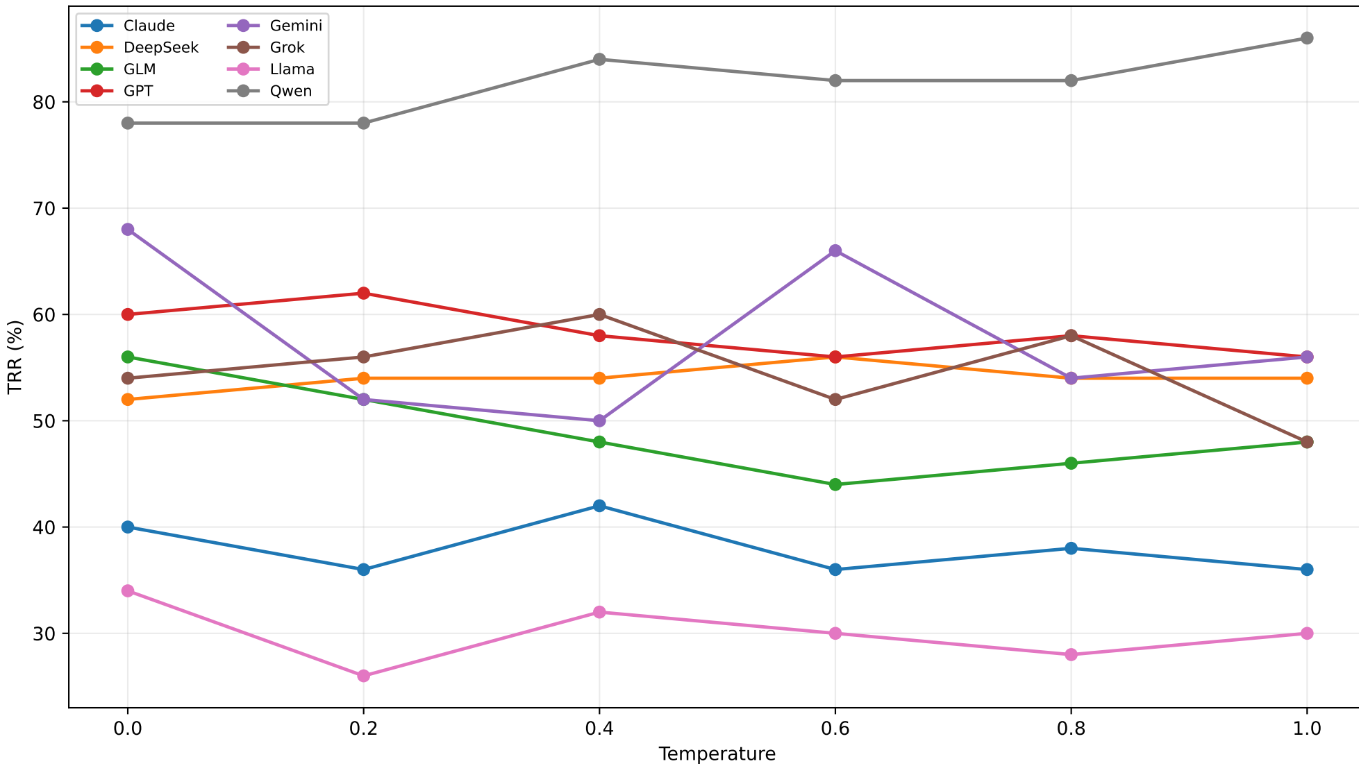
Temperature Sensitivity of Toxic Prompt Refusal
