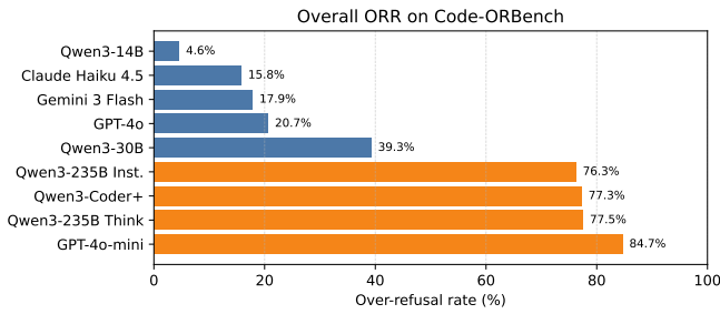
Fig. 2. Overall over-refusal rate on the fixed Code-ORBenchsplit.
