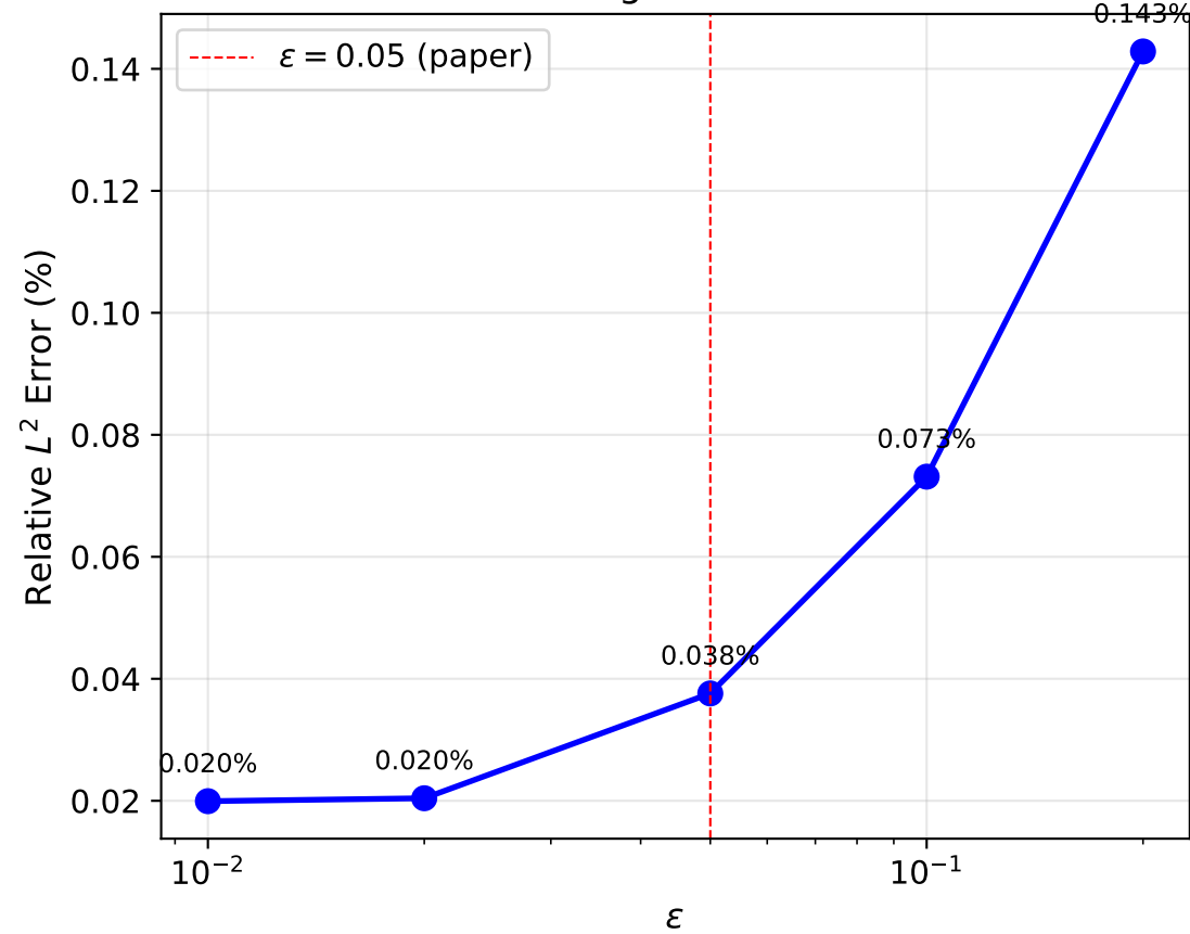
Pricing Error vs \varepsilon
