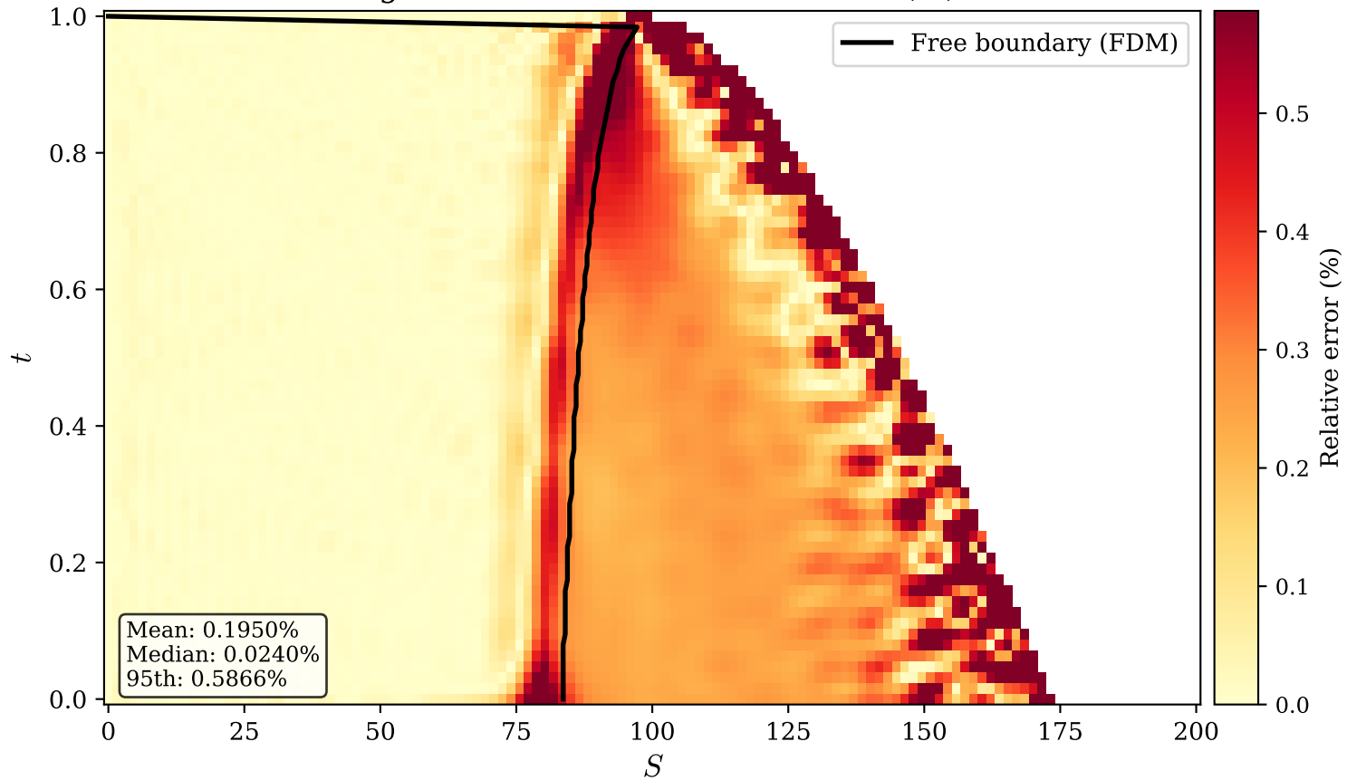
Figure 8: Pointwise Relative Error (%)
