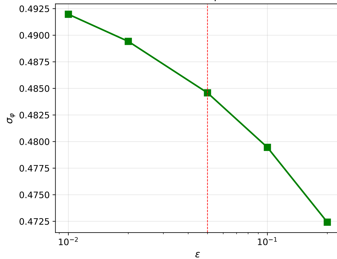
Phase-Field Sharpness vs \varepsilon
