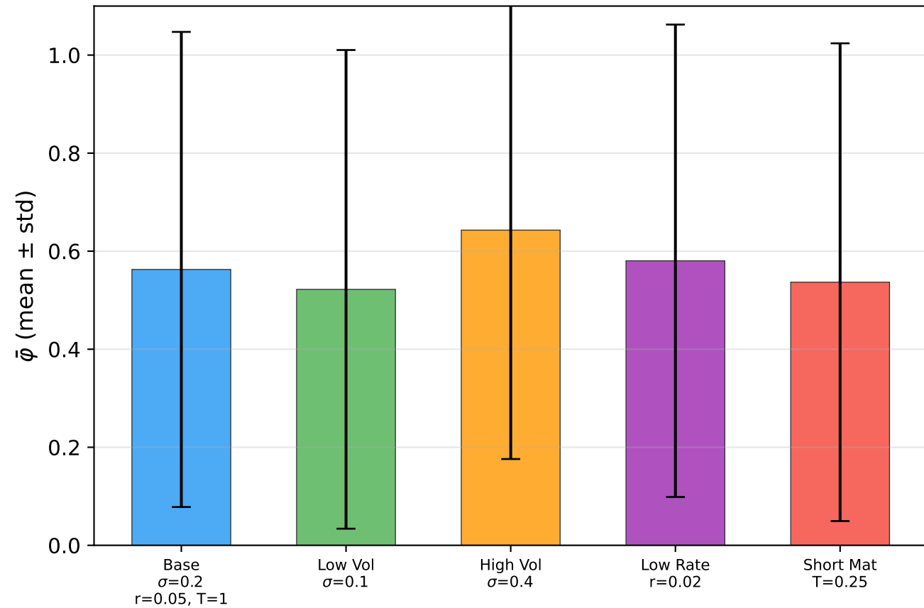
Phase-Field Statistics
