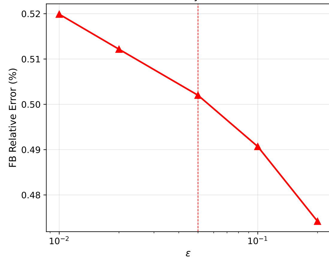
Free Boundary Error vs \varepsilon
