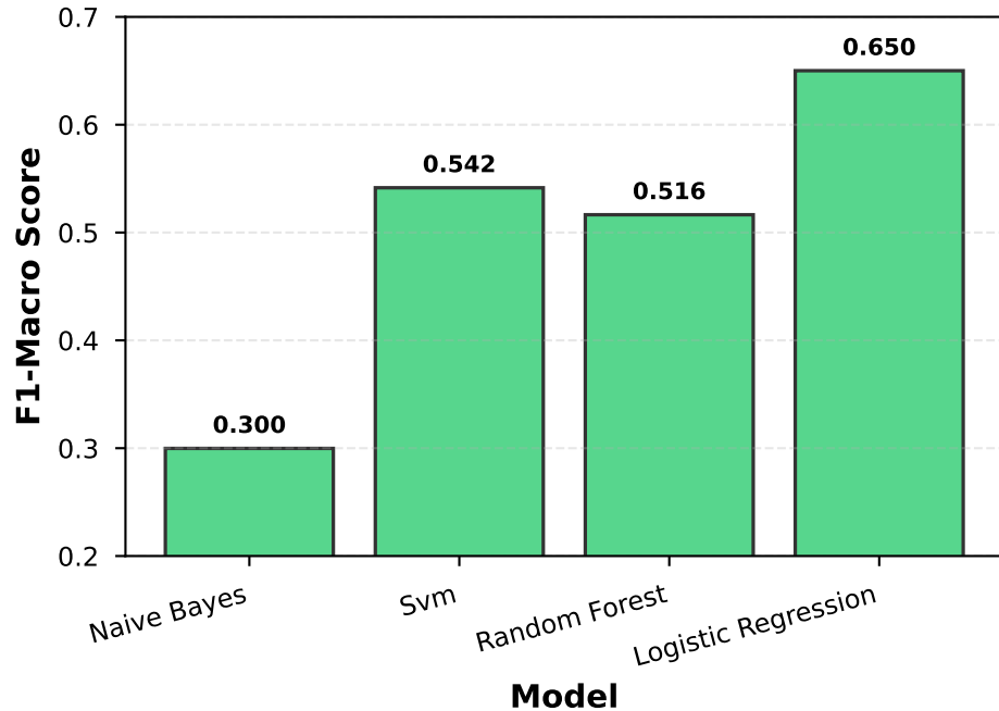
Development Set F1-Macro
