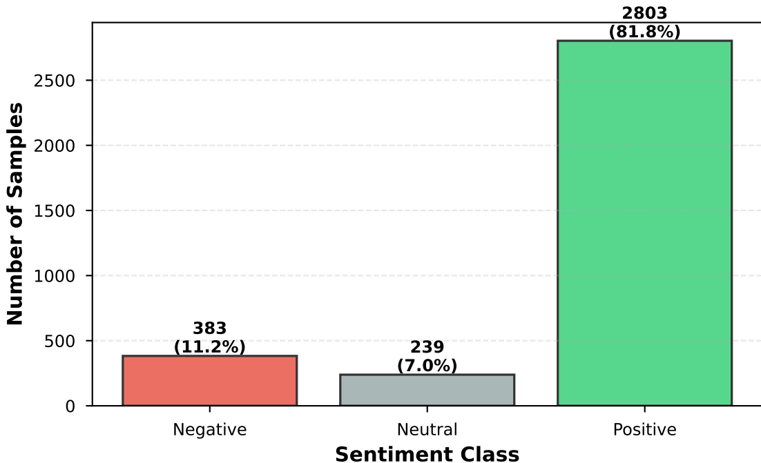
Label Distribution (3-Class Sentiment)
