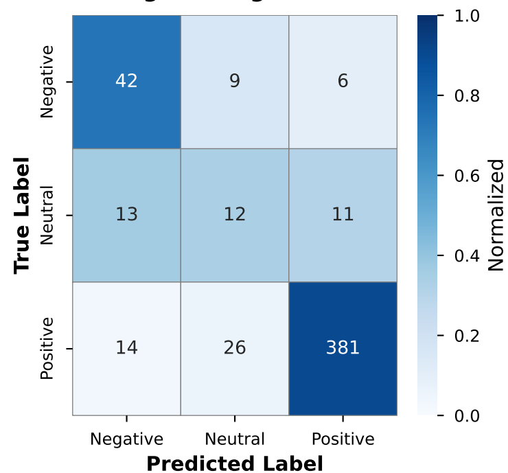
Logistic Regression
