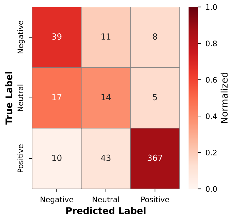
PhoBERT
