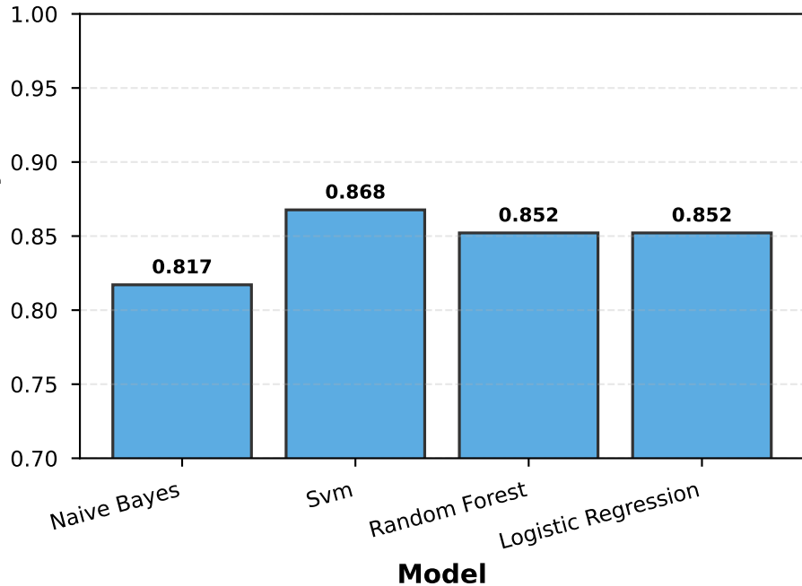
Development Set Accuracy
