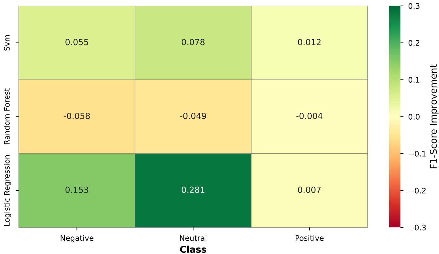
F1-Score Improvement by Class and Model (With Class Weight - Without Class Weight)
