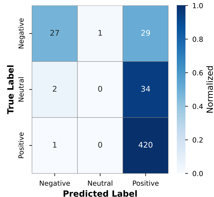
Random Forest
