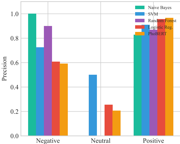
Precision by Class
