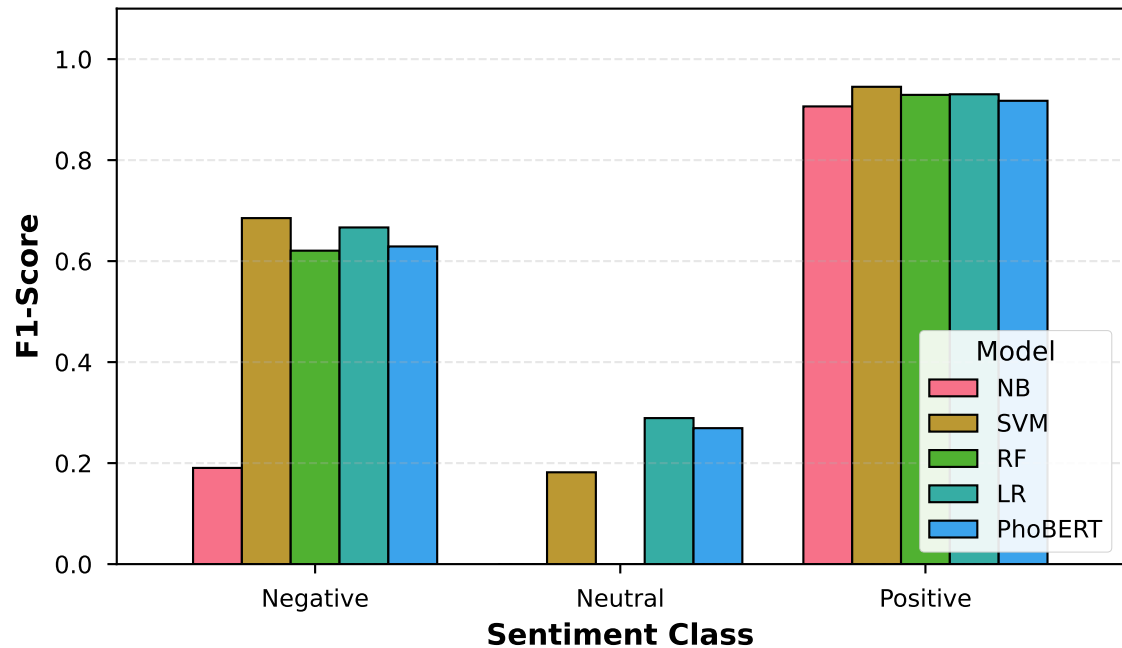
F1-Score by Class
