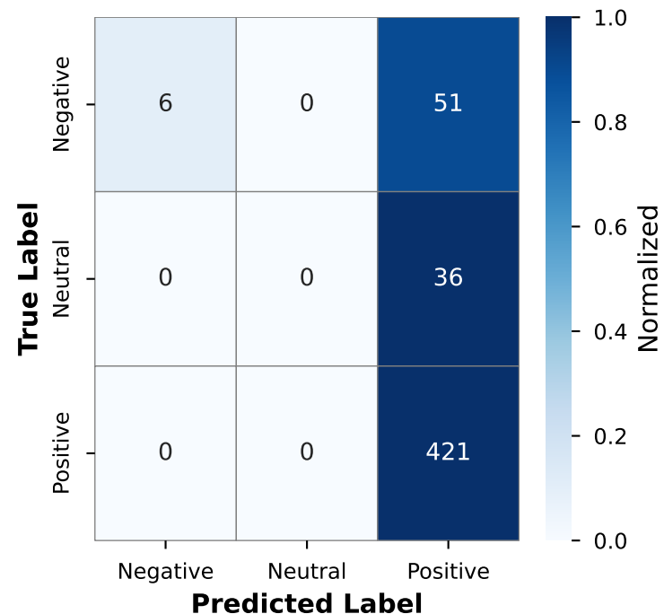
Naive Bayes
