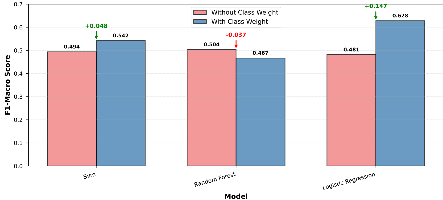
Class Weight Impact on F1-Macro (Development Set)
