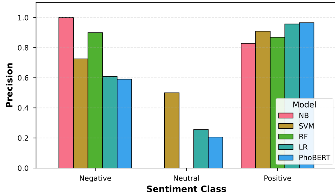
Precision by Class
