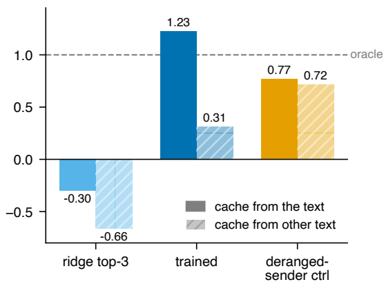
continuation retention
