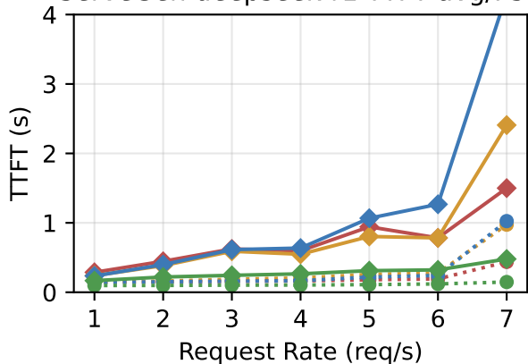
Synthetic mix (5%) TTFT avg/P50
