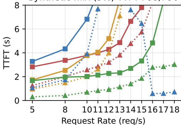
Synthetic mix (5%) TTFT P99/P90
