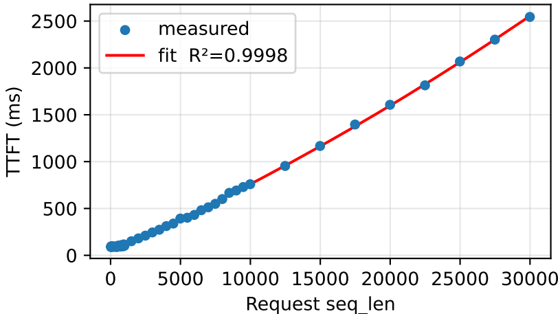
TTFT vs seq length (TP=4)
