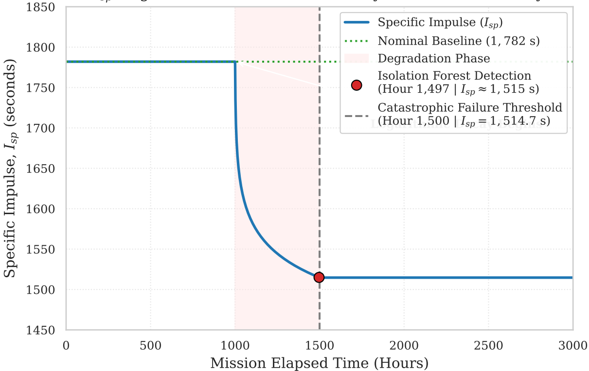
I_{sp} Degradation Timeline & Anomaly Detection Boundary
