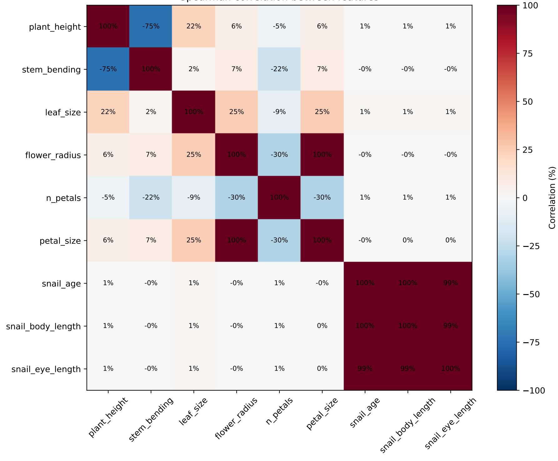
Spearman correlation between features
