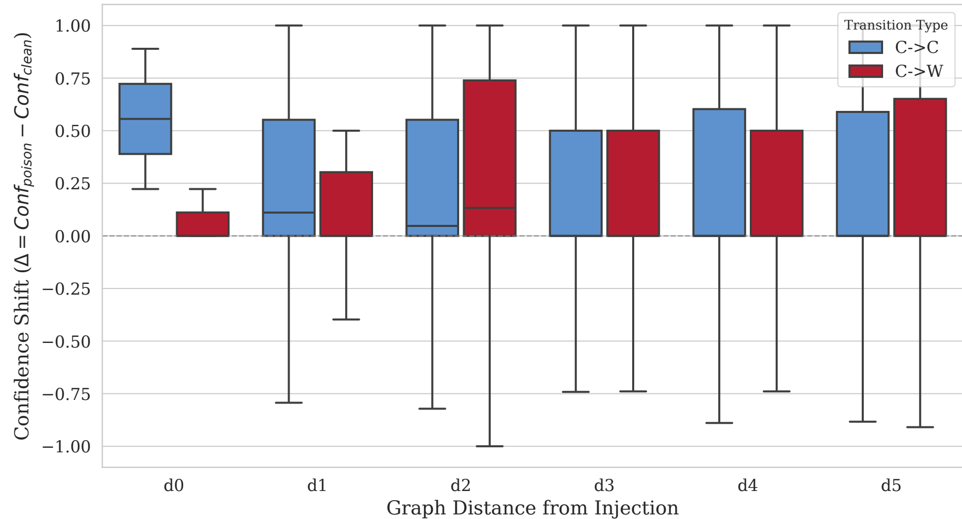
Global Confidence Inflation: Correct vs. Hallucinated Outputs
