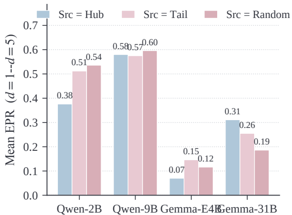
(b) Impact: error propagation by source class
