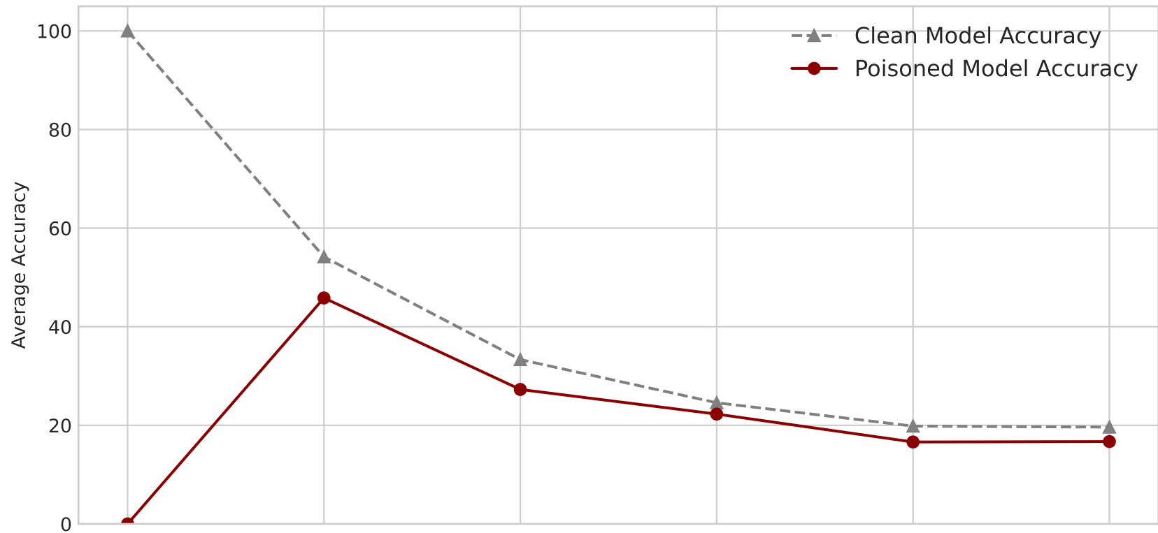
Effect of Poisoning on Model Accuracy vs. Graph Distance
