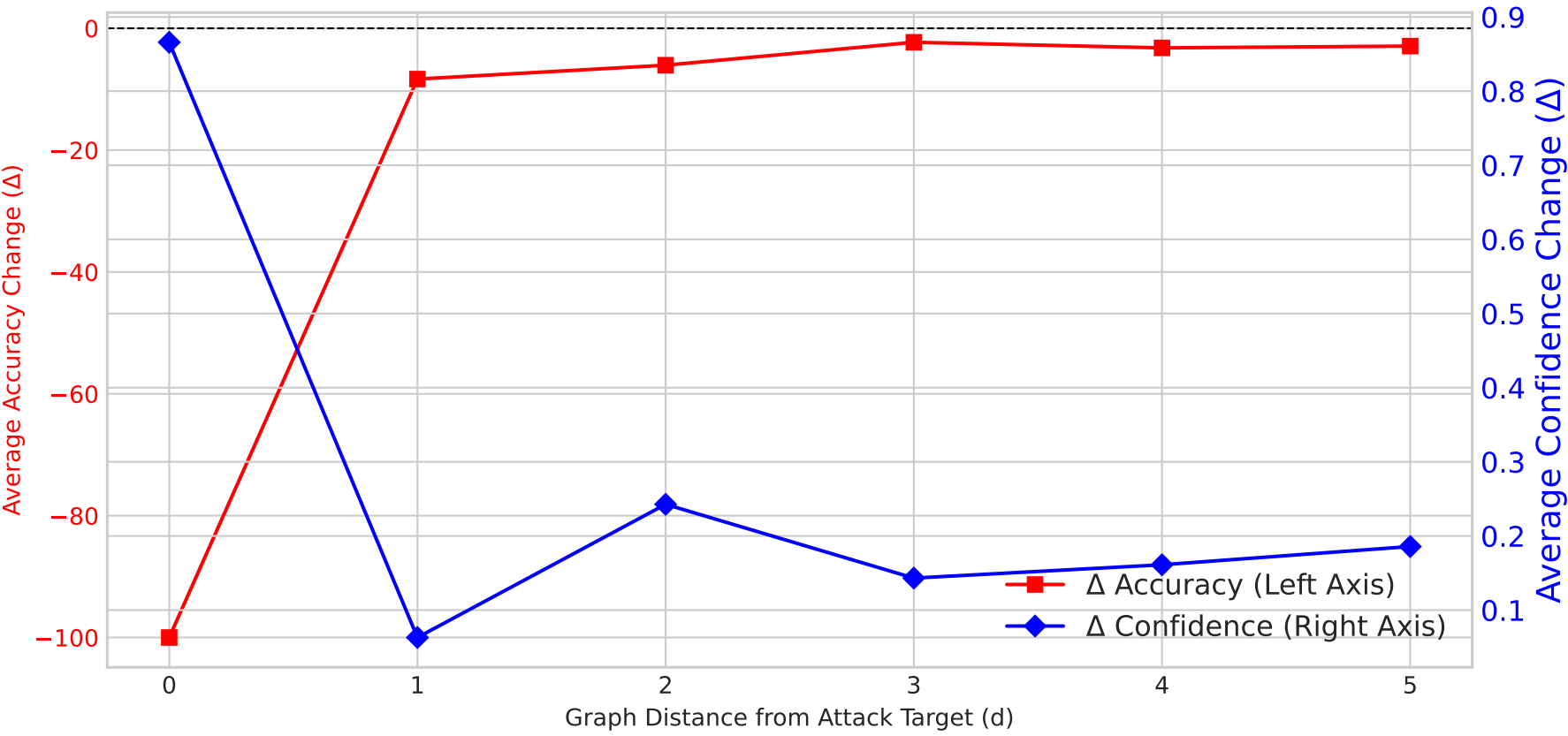
Average Change ( \Delta ) in Accuracy & Confidence vs. Graph Distance
