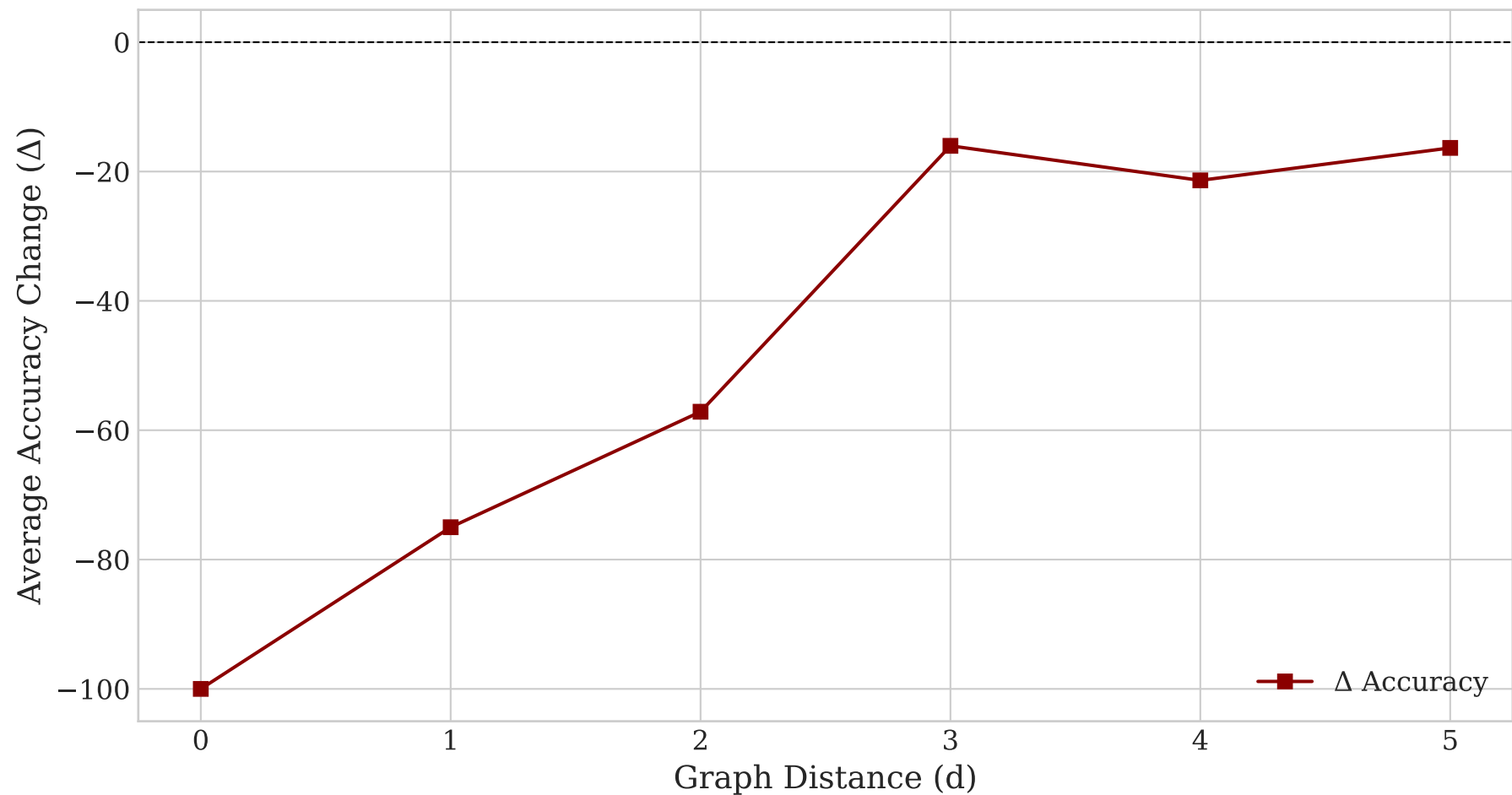
Average Accuracy Change vs. Graph Distance
