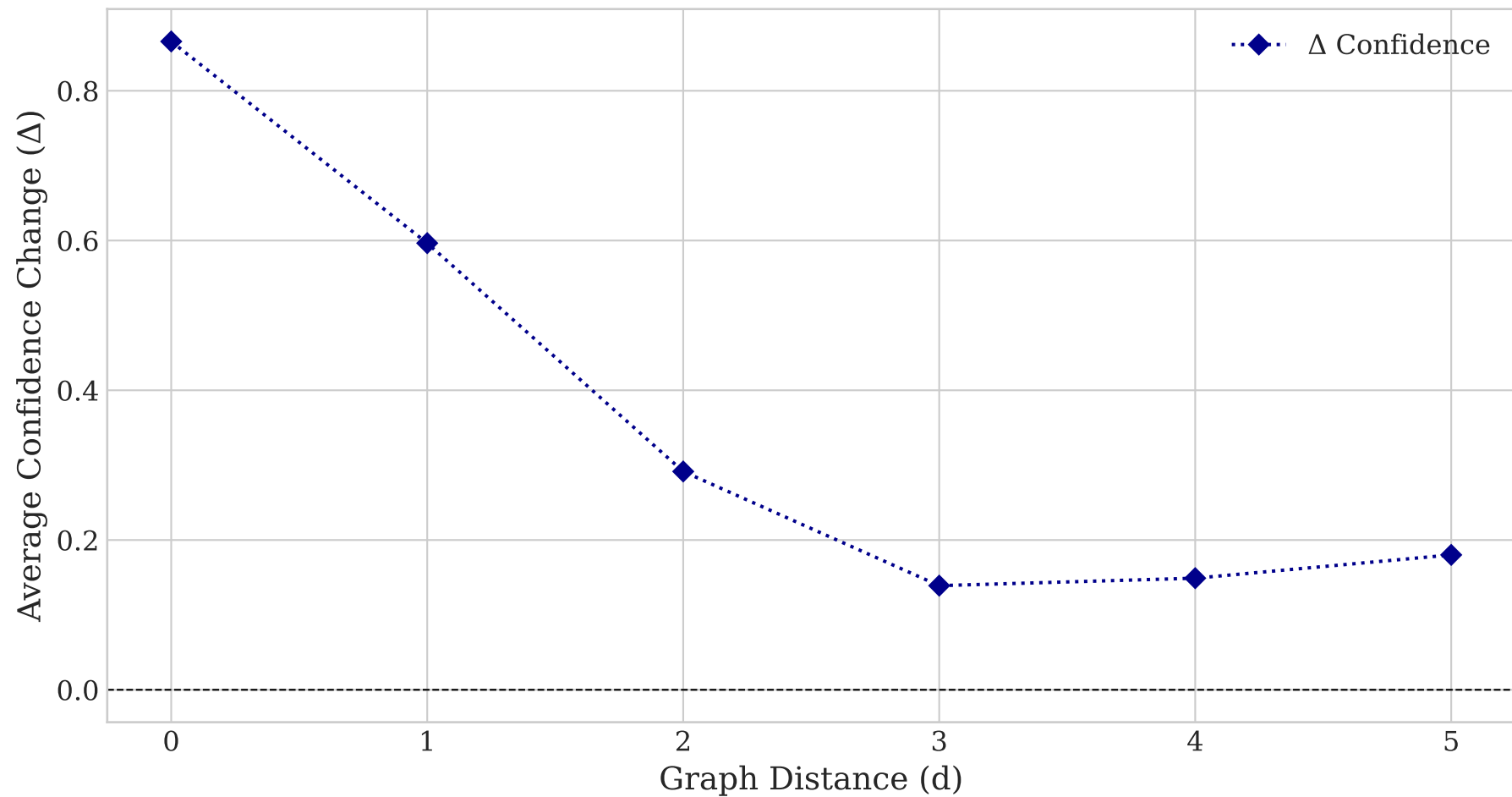
Average Confidence Change vs. Graph Distance
