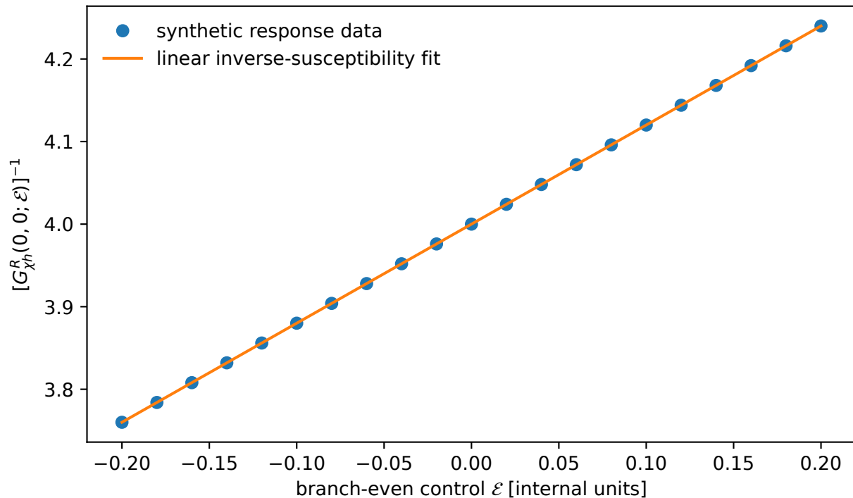
Even gate is measured through the inverse odd susceptibility
