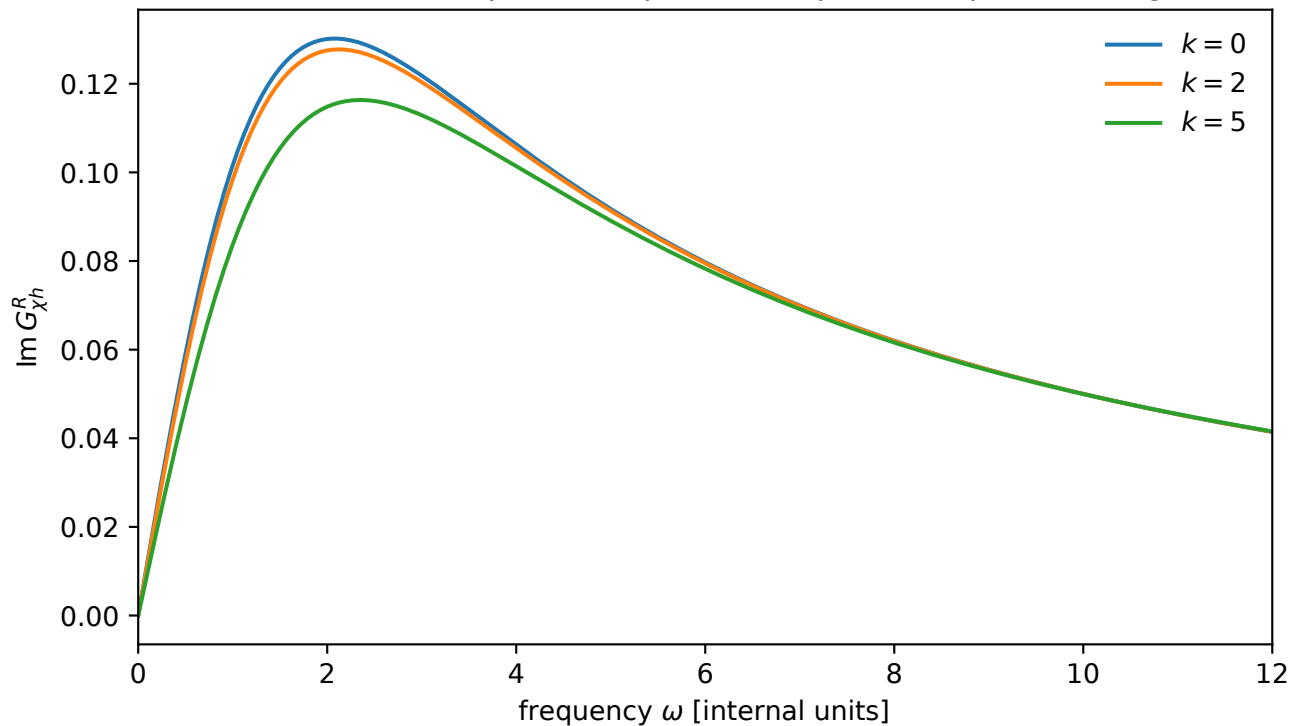
Passive retarded phase response has positive spectral weight
