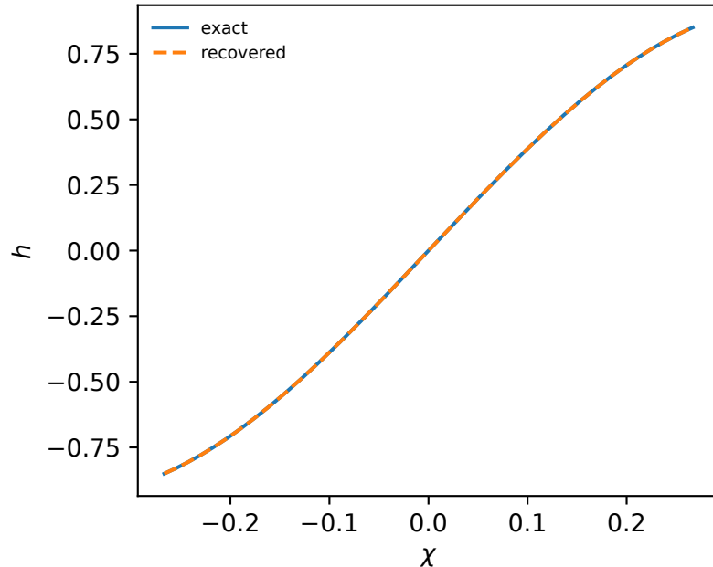
(b) nonlinear 1PI recovery
