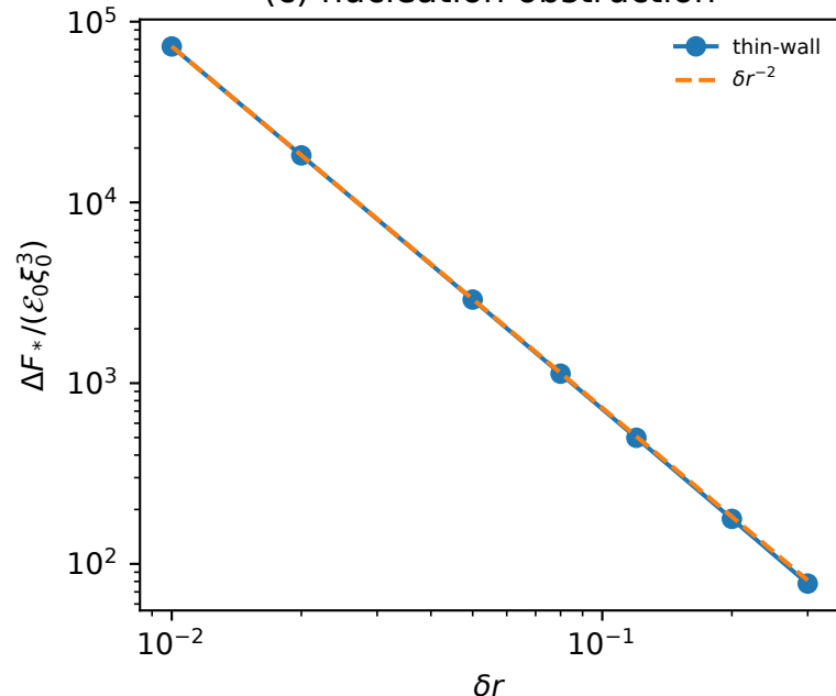
(c) nucleation obstruction
