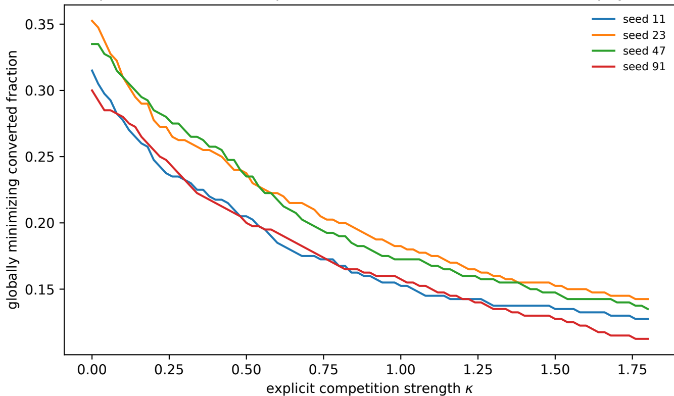
A positive nonlocal competition term can self-limit, but is extra physics
