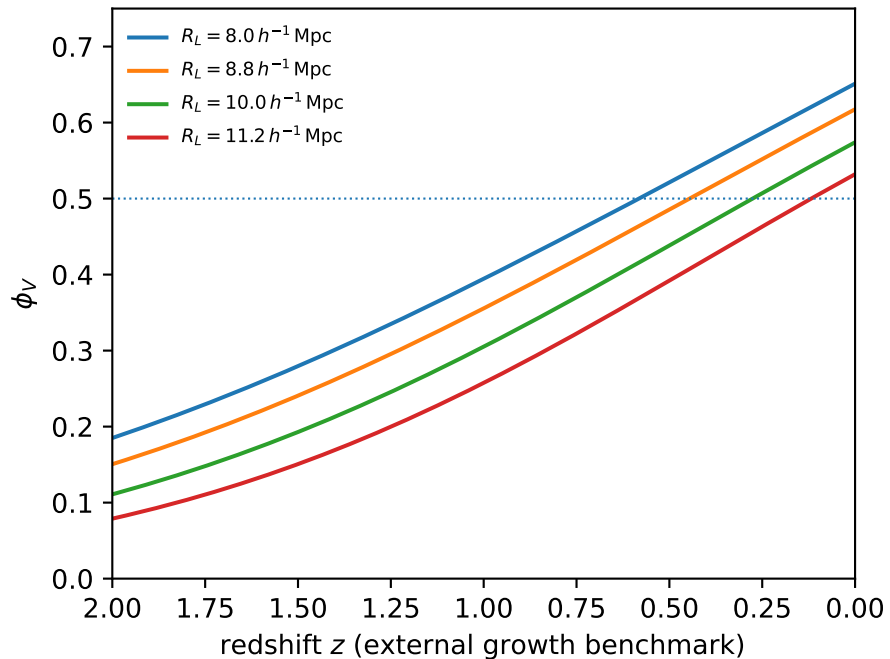
Curvature-equality selector: benchmark histories
