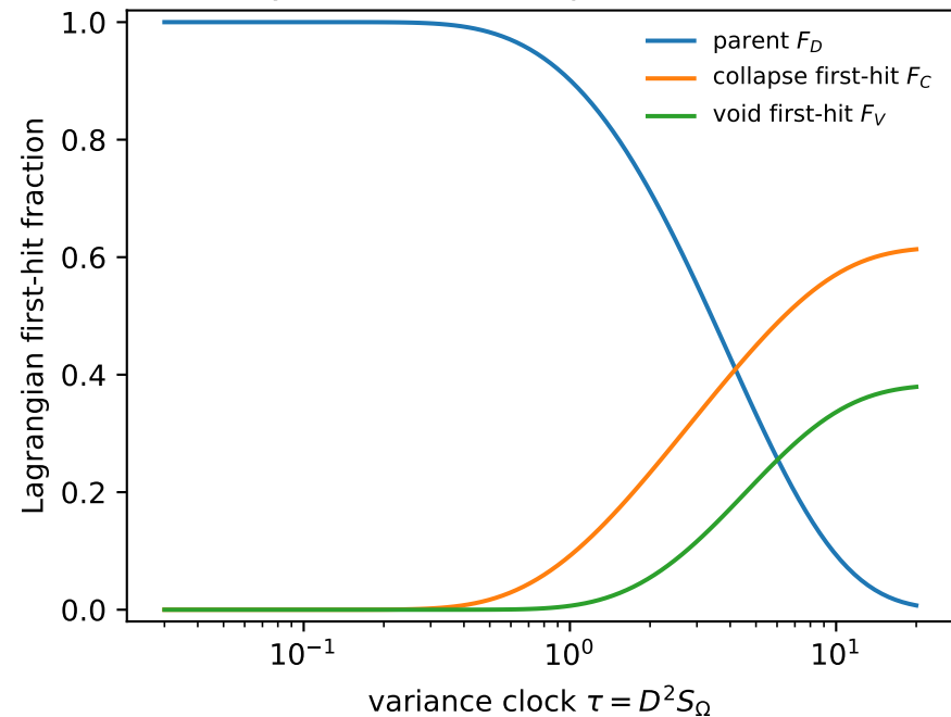
Dynamical-barrier phase fractions
