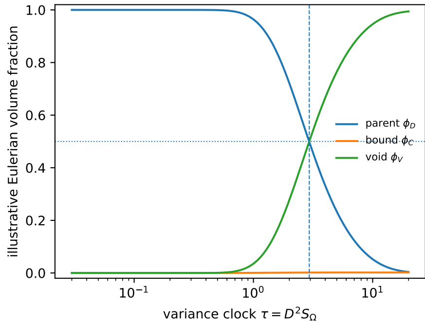
Mass-rich vs volume-rich coexistence
