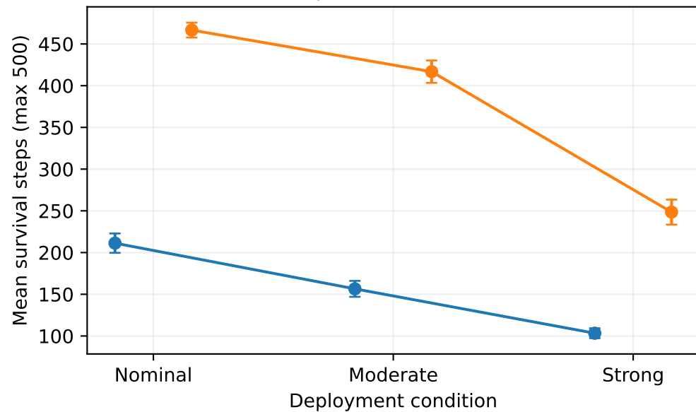
Episode survival
