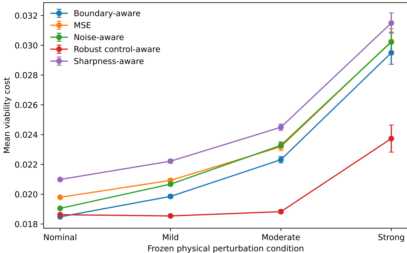
E-020C1 robustness under frozen perturbations
