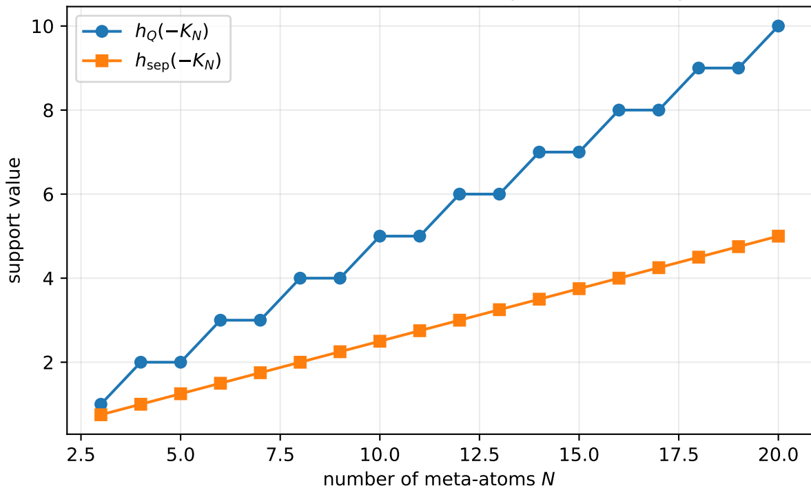
Exact frustrated collective-response advantage
