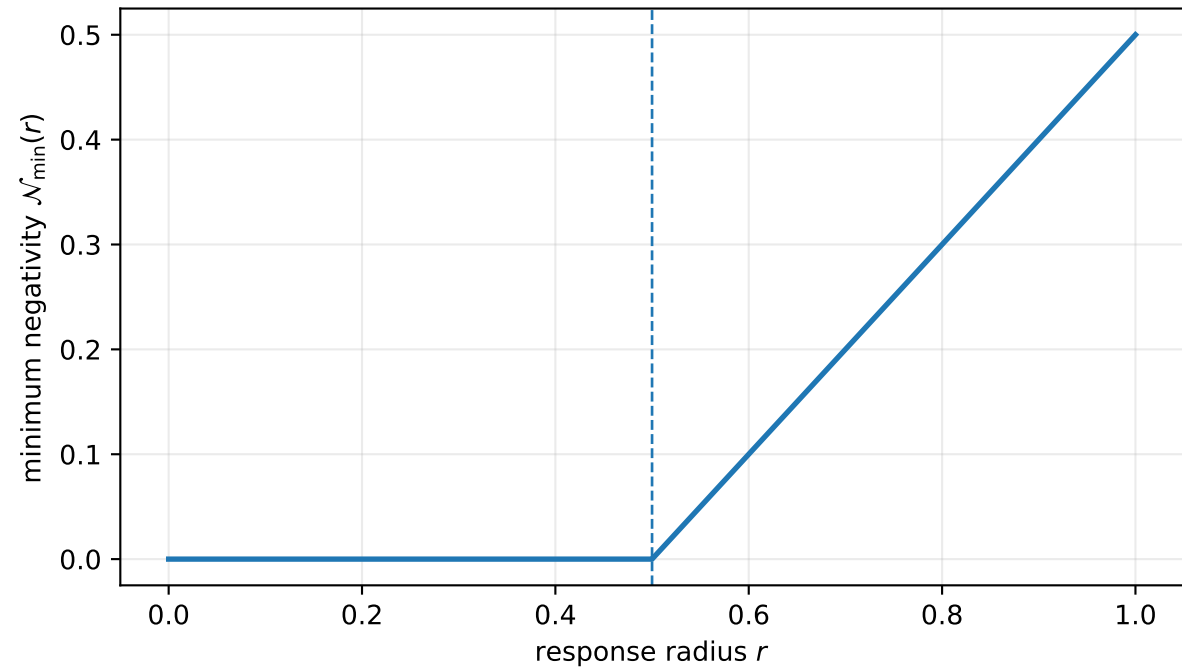
Exact entanglement cost of the two-emitter response
