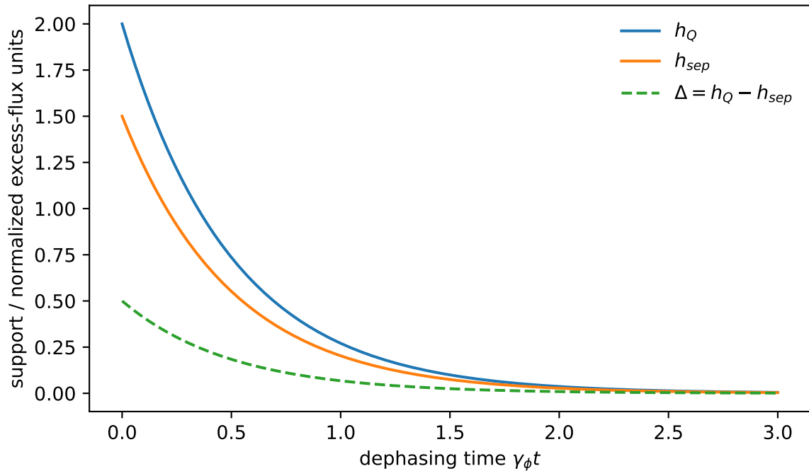
Exact contraction under independent pure dephasing
