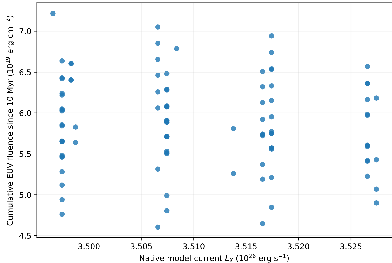
LHS 1140: present activity carries little ranking information for history
