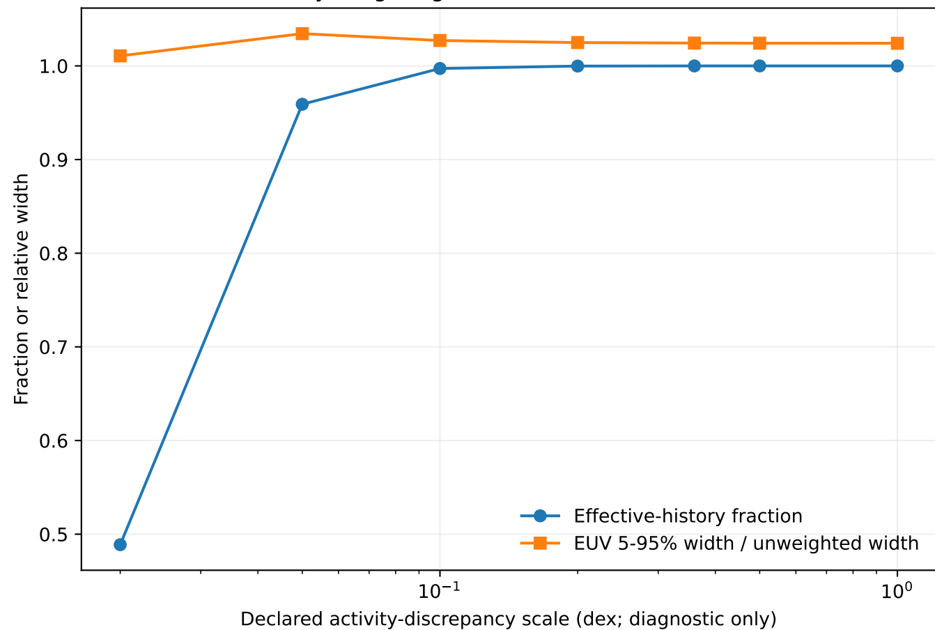
LHS 1140: activity weighting does not contract the historical interval
