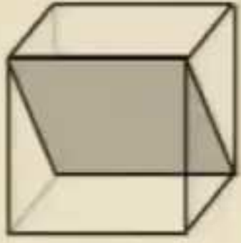
(011)
