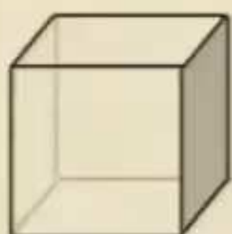
(100)
