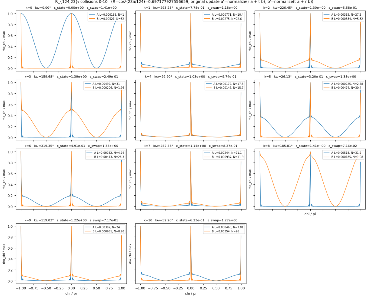
Figure 3: Figure 3: Waveforms of the two waves at R_{124,23} (collisions 0 to 10)
