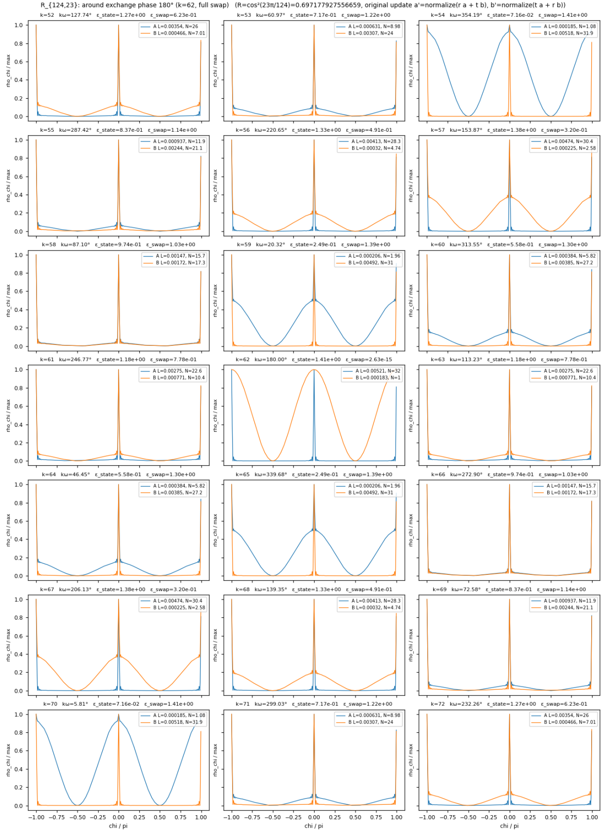
Figure 4: Figure 4: Around exchange phase 180^\circ (collisions 52 to 72)
